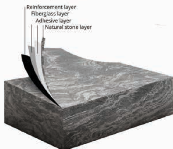
Composite layers of Stonex Veneer
